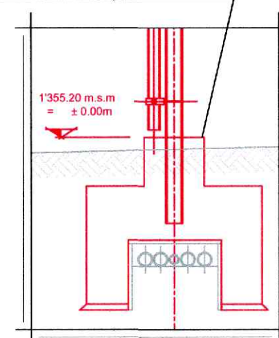
DETAIL POINT ZERO
