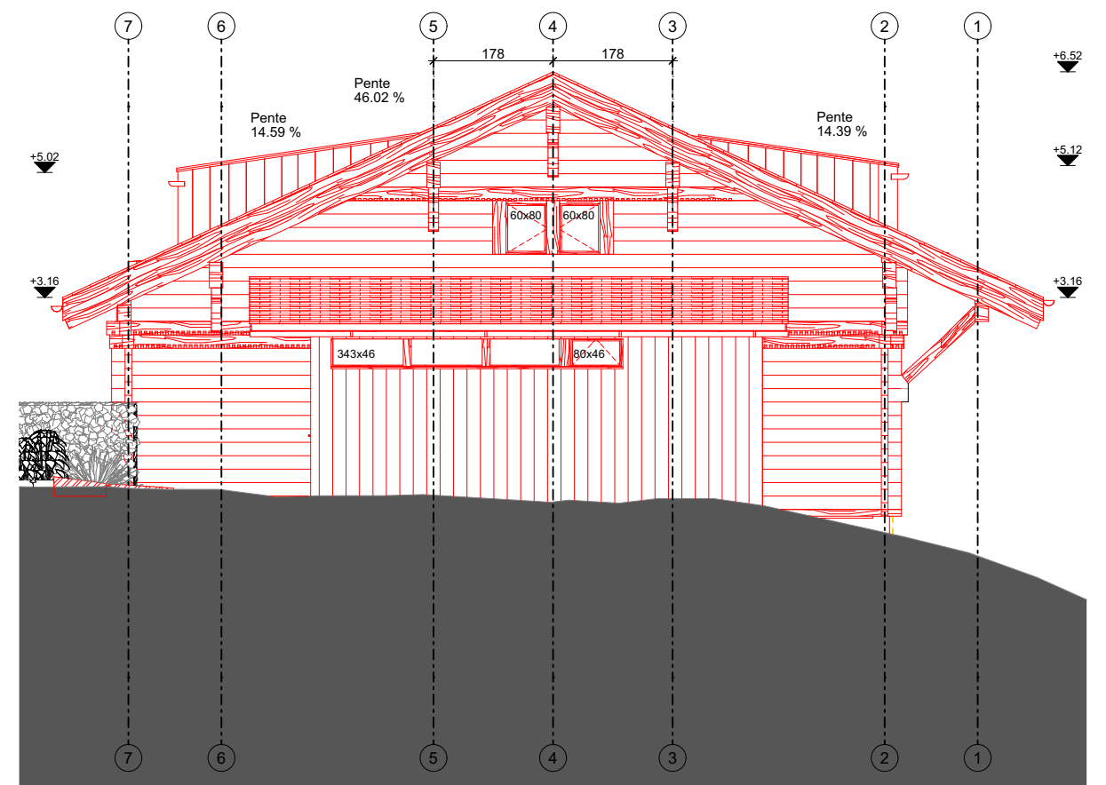
Façade N-E
