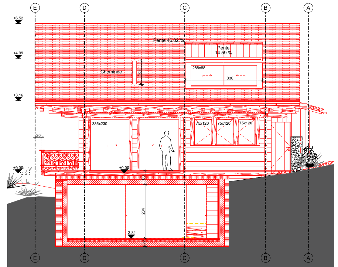
Façade S-E
